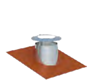
Flashing kit 5-15° with FastFlash plate elastomer red and storm collar
