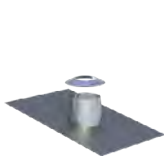
Flashing kit 5-15° lead base with storm collar, cone 150mm
